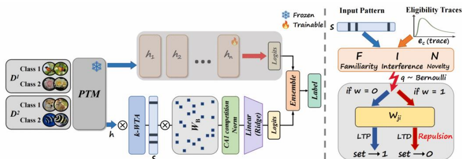
Figure 1. Illustration of BTSP-CAM. Left: Overall architecture, where a frozen PTM provides semantic features and a parallel BTSP-CAM branch converts them into sparse RF codes, stores them in a binary memory W_B , and produces CA1 logits via competition and ridge consolidation that can be ensemble with the PTM head. Right: Synaptic update mechanism, in which familiarity, interference, and novelty signals derived from the input code and eligibility traces gate BTSP-style bit flips, so that LTP ( 0 \rightarrow 1 ) allocates new patterns while collision-aware LTD ( 1 \rightarrow 0 ) repels conflicting ones in Hamming space.
